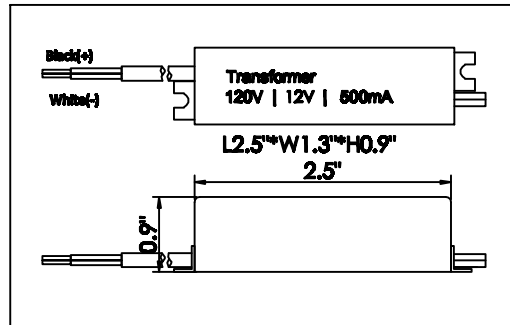
Electronic Transformer DIAGRAM
